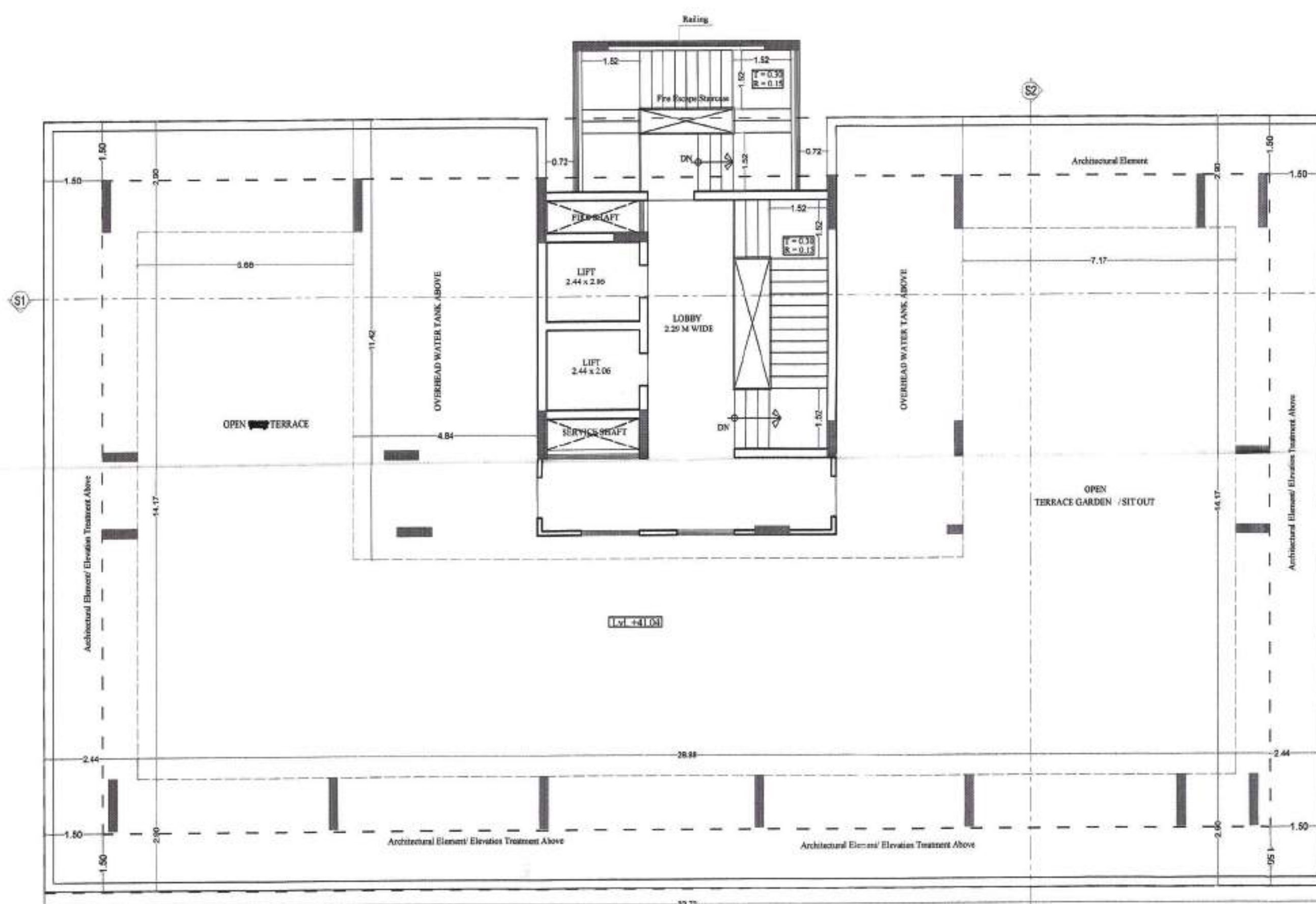
TERRACE PLAN
