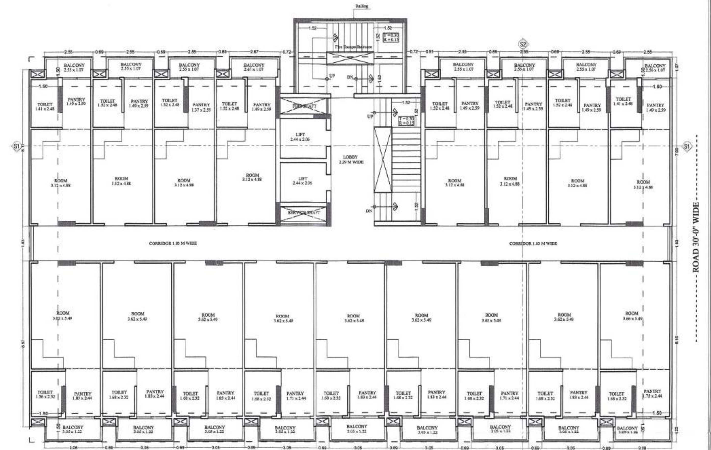
TYPICAL PLAN (2nd to 12th Floor)
